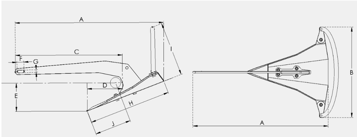
M1 MODEL DIMENSIONS (IMPERIAL)
